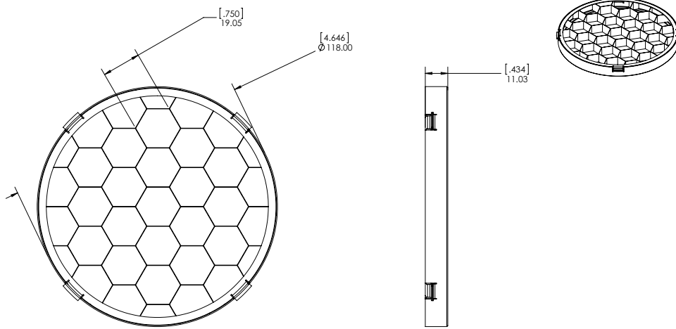
45° Cutoff Hex Louver (Requires 55° cutoff short snoot)
