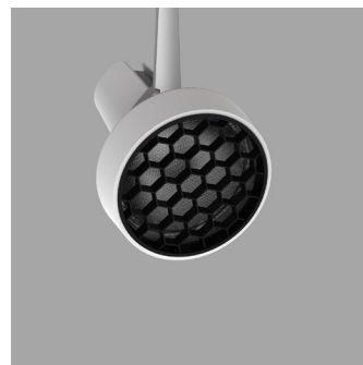
45° Cutoff Hex Louver with 55° Cutoff Short Snoot
