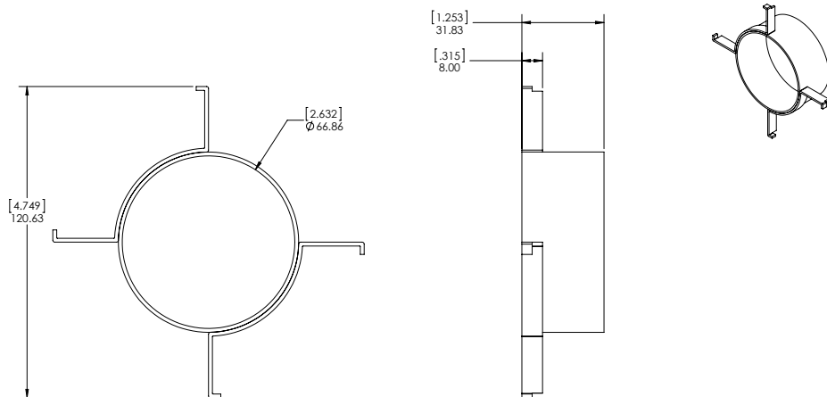
10° Cutoff Baffle (Requires 30° cutoff tall snoot)
